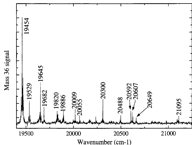
FIG. 1. Vibronically resolved scan of the \tilde{B}^2\Pi_g-\tilde{X}^2\Sigma_u^+ band system of ^{11}\text{B}^{14}\text{N}^{11}\text{B} . Wave numbers of the major features are given.
