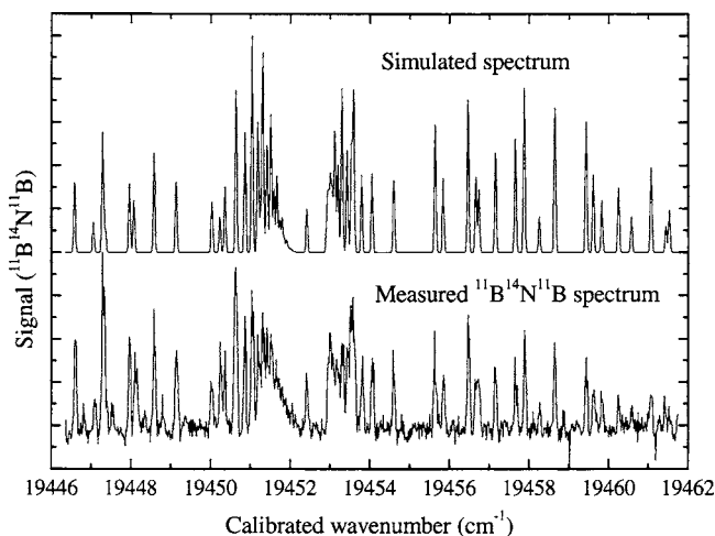
FIG. 2. Rotationally resolved scan over the central portion of the origin band of the \tilde{B}^2\Pi_g-\tilde{X}^2\Sigma_u^+ band system of ^{11}\text{B}^{14}\text{N}^{11}\text{B} (lower panel) and the simulated spectrum (upper panel). Nuclear spin statistics for identical I=3/2 ^{11}\text{B} nuclei are included in the simulated spectrum.
