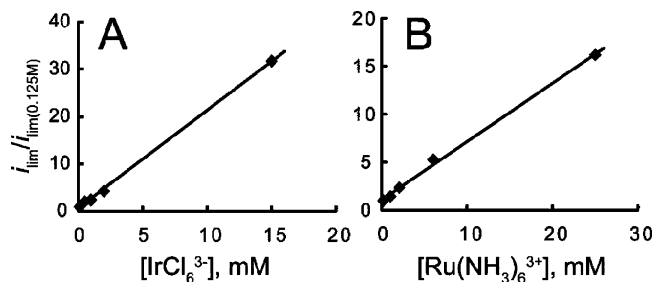
Figure 7. Relative limiting current of sulfonated colloidal film electrodes as a function of concentration of (A) IrCl_6^{3-} and (B) Ru(NH_3)_6^{3+} in water.
