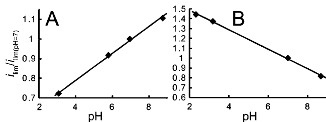
Figure 5. Relative limiting current of the sulfonated colloidal film electrodes as a function of pH for \text{Ru}(\text{NH}_3)_6^{3+} (A) and for \text{IrCl}_6^{3-} (B).
